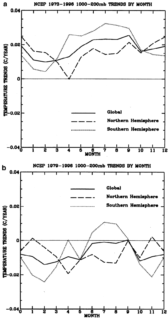
Figure 2. Global and northern and southern hemisphere monthly 1000-200 mbar layer temperature trends ( ^{\circ}\text{C yr}^{-1} ) calculated from the NCEP reanalysis for (a) 1973-1996 and (b) 1979-1996. Months are plotted along the x axis (0 = December, 1 = January, ..., 12 = December).
