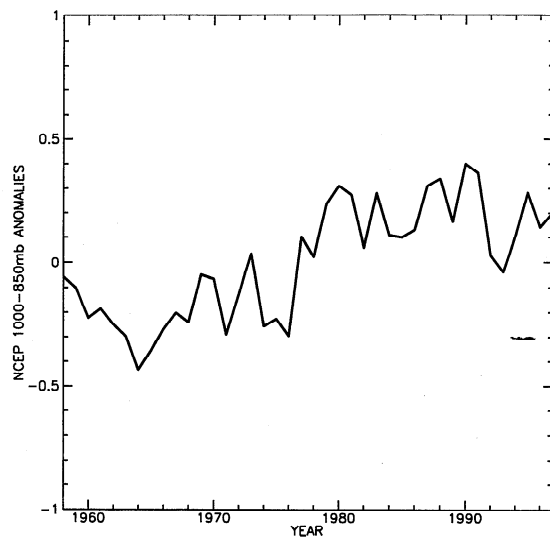
Figure 5. NCEP 1958-1997 global layer temperature anomaly ( ^{\circ}\text{C} ) time series for 1000-850 mbar defined with respect to the 40-year climatology.
