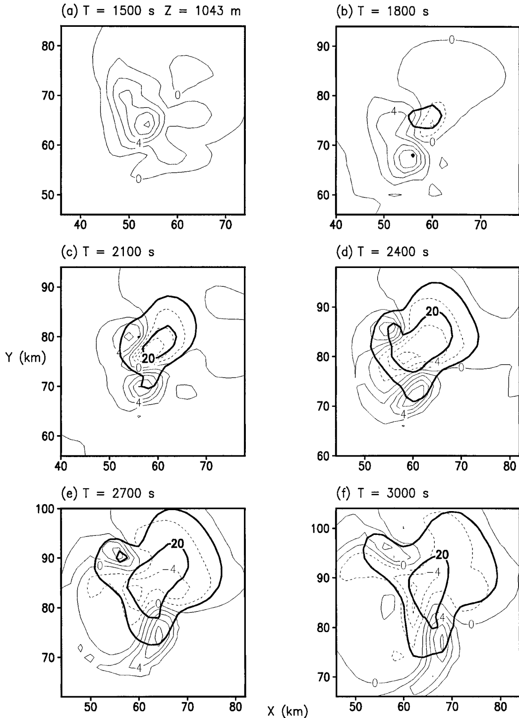
FIG. 7. Vertical motion (contoured every 2 \text{ m s}^{-1} ), thin contours, along with (-\theta_0 \partial \pi^* / \partial z) \times 10^2 (contoured every 10 \text{ m s}^{-2} ), thick contours, from (a) 1500, (b) 1800, (c) 2100, (d) 2400, (e) 2700, and (f) 3000 s at 1043 m.
