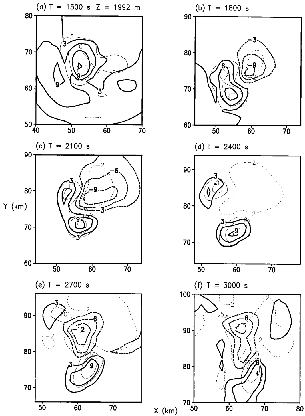
FIG. 5. Vertical motion (contoured every 5 \text{ m s}^{-1} ), thin contours, along with \{[(\theta_v - \theta_0)/\theta_0 - r_c]g\} \times 10^2 (contoured every 3 \text{ m s}^{-2} ), thick contours, from (a) 1500, (b) 1800, (c) 2100, (d) 2400, (e) 2700, and (f) 3000 s at 1992 m.
