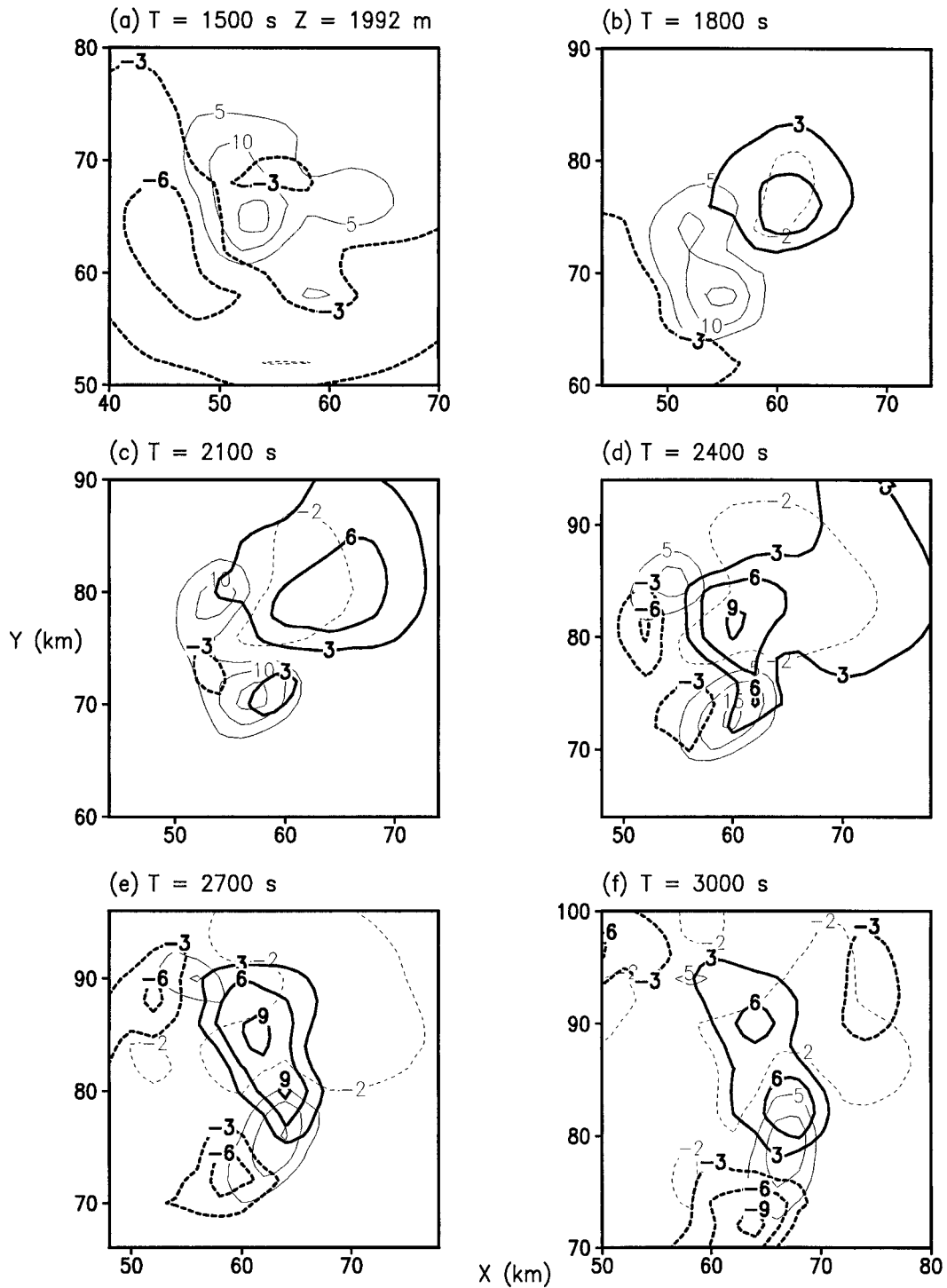
FIG. 4. Vertical motion (contoured every 5 m s -1 ), thin contours, along with (-\theta_0 \partial \pi^* / \partial z) \times 10^2 (contoured every 3 m s -2 ) thick contours, from (a) 1500, (b) 1800, (c) 2100, (d) 2400, (e) 2700, and (f) 3000 s at 1992 m.
