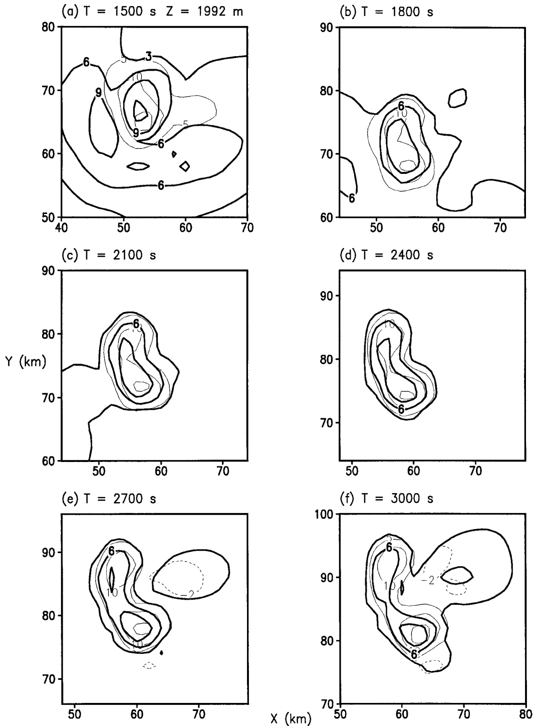
FIG. 13. Same as Fig. 5 for the no-precipitation simulation.
