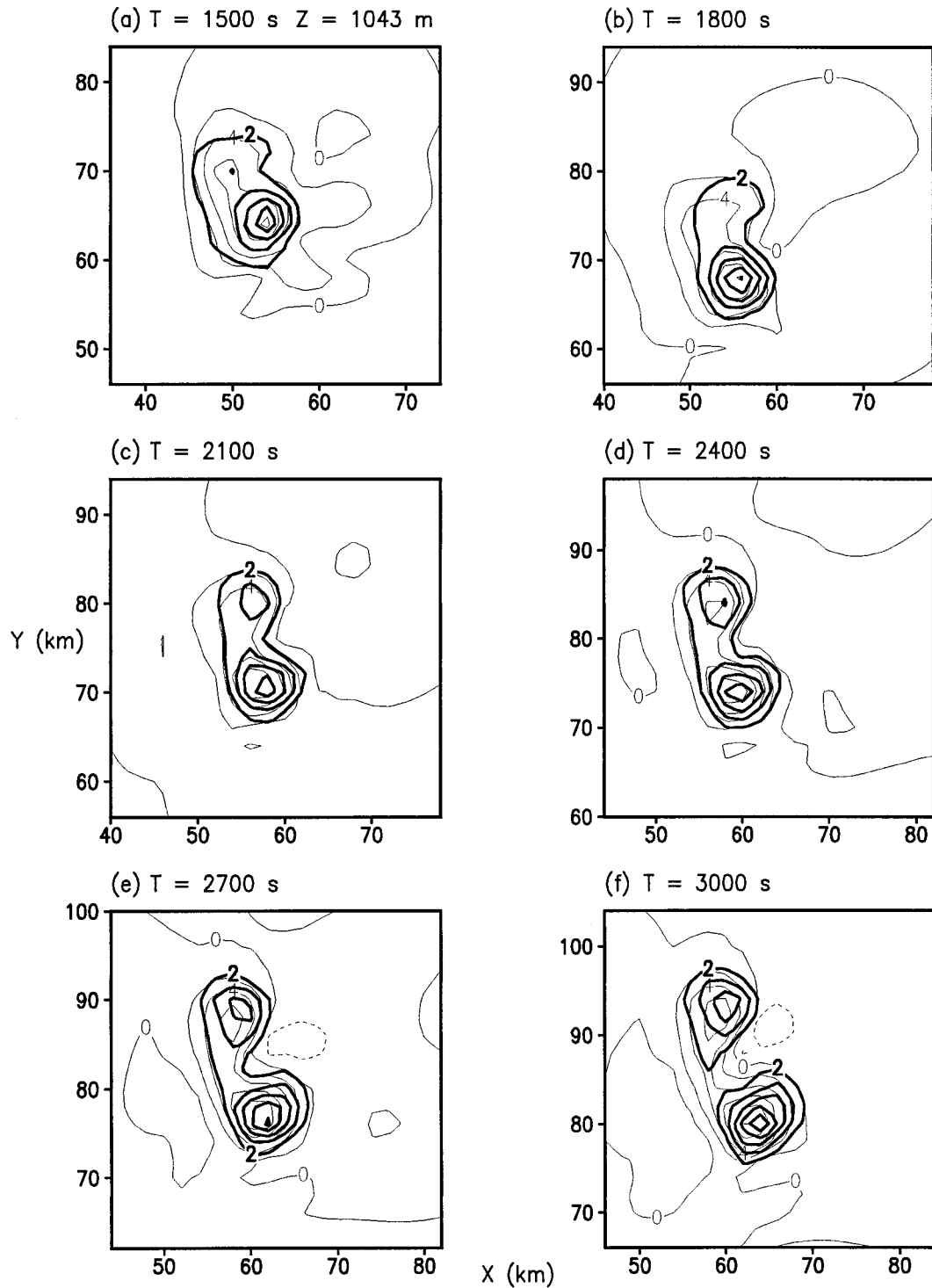
FIG. 14. Vertical motion (contoured every 2 \text{ m s}^{-1} ), thin contours, along with \{-\theta_0 \partial \pi^* / \partial z + [(\theta_v - \theta_0) / \theta_0 - r_c] g\} \times 10^2 (contoured every 2 \text{ m s}^{-2} ), thick contours, from (a) 1500, (b) 1800, (c) 2100, (d) 2400, (e) 2700, and (f) 3000 s at 1043 m.
