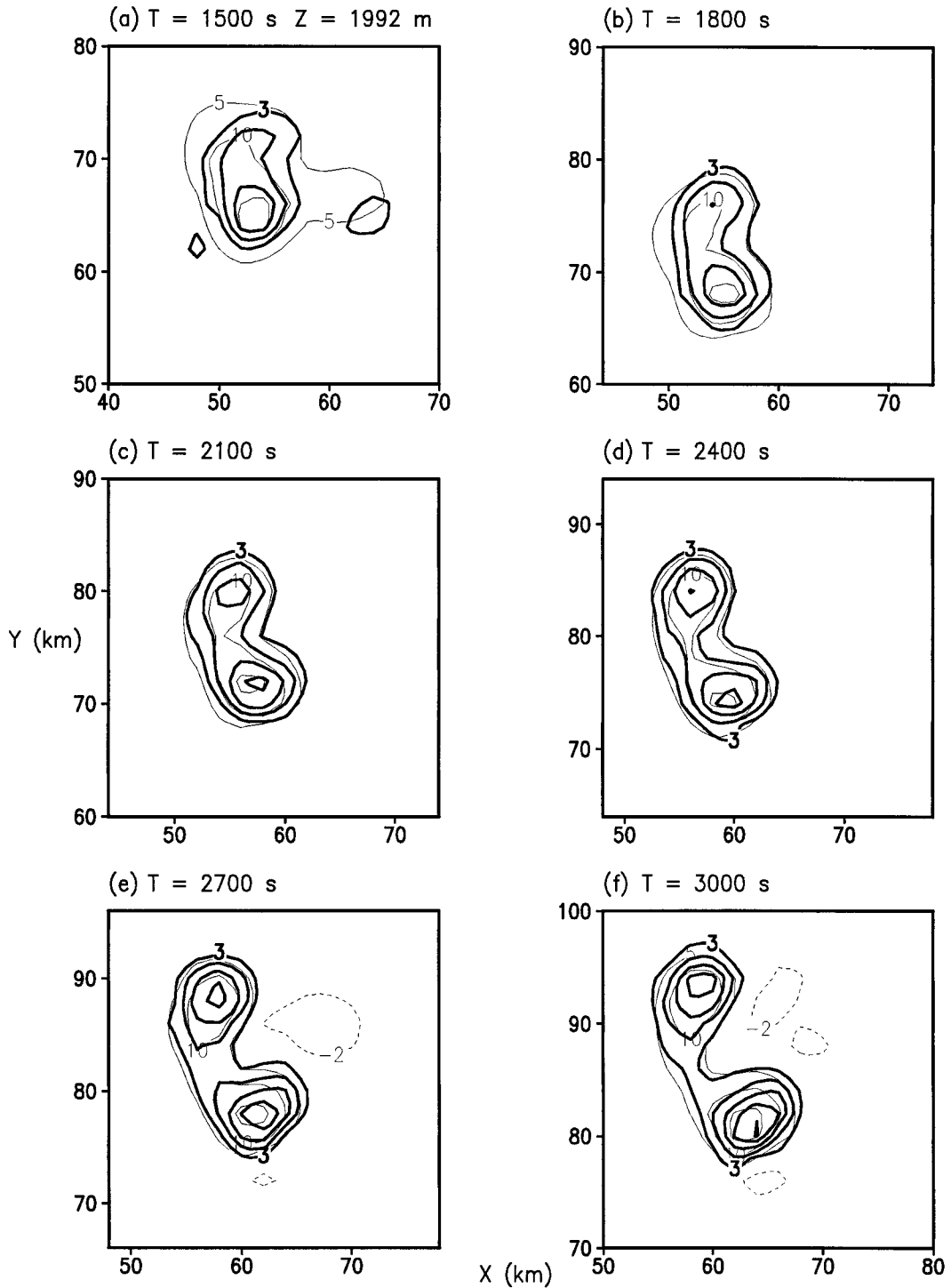
FIG. 11. Same as Fig. 3 for the no-precipitation simulation.
