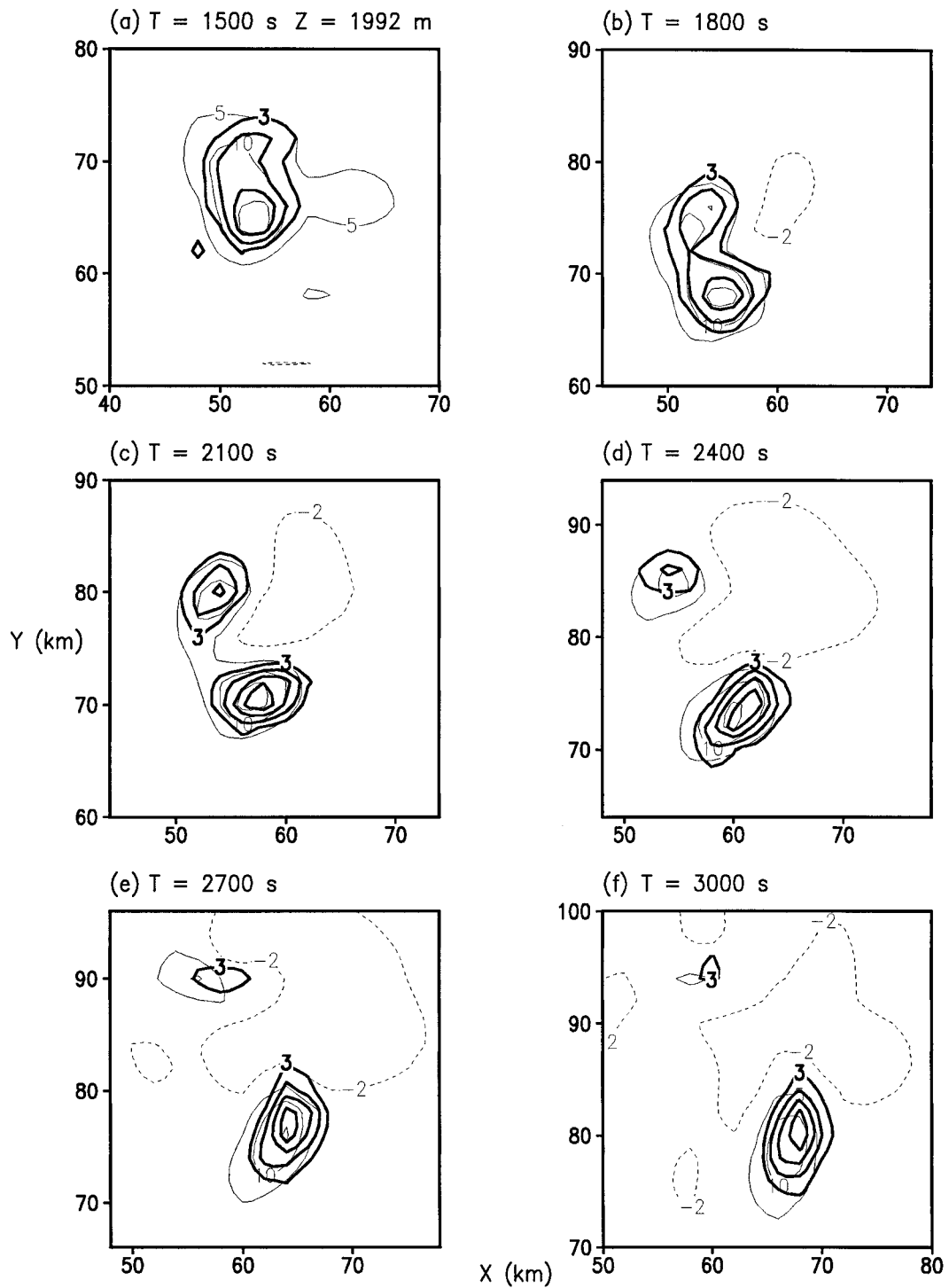
FIG. 3. Vertical motion (contoured every 5 \text{ m s}^{-1} ), thin contours, along with \{-\theta_0 \partial \pi^* / \partial z + [(\theta_v - \theta_0) / \theta_0 - r_c] g\} \times 10^2 (contoured every 3 \text{ m s}^{-2} ), thick contours, from (a) 1500, (b) 1800, (c) 2100, (d) 2400, (e) 2700, and (f) 3000 s at 1992 m.
